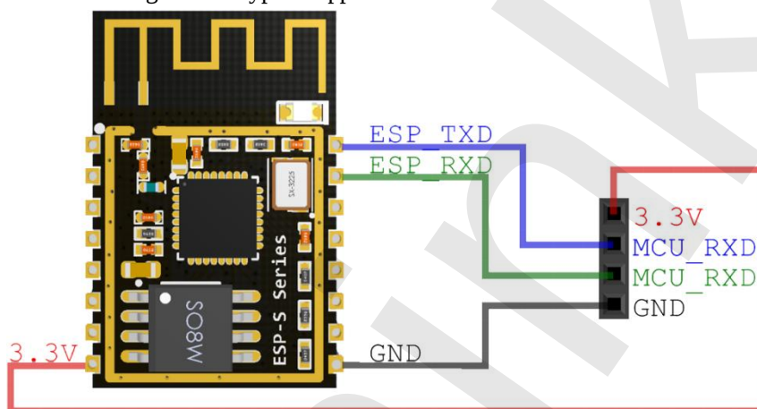
Figure 4.7 Typical application of ESP-12S
