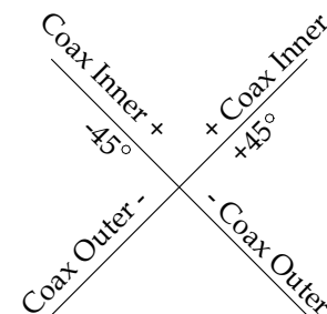
Rear view of the Antenna dipoles
