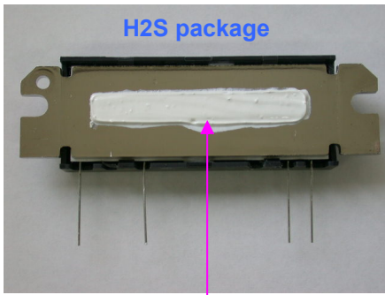
Thermal compound size: L40 x W6.0 x t 0.5mm
